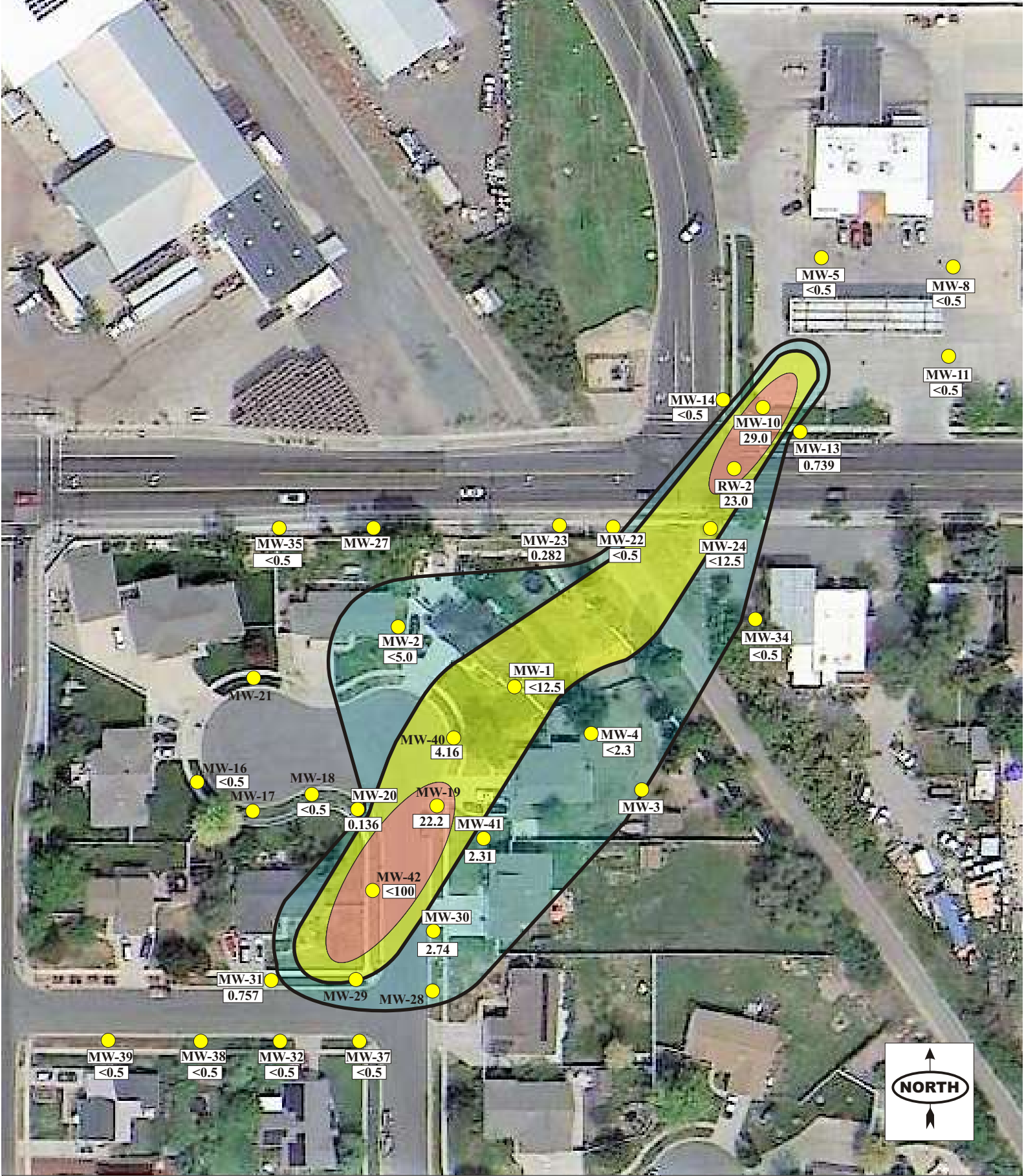
Triple Stop Chevron 1034 W Gentile Street Layton, Utah Figure 4 Dissolved TPH January 2022
